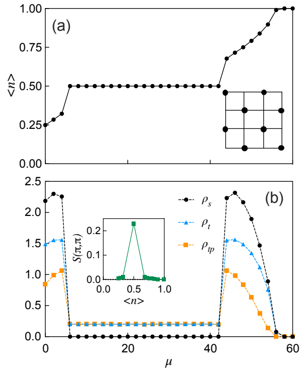
FIG. 7. The boson density (a) and the various stiffness constants (b) as functions of \mu . The inset of (a) illustrates the geometry of bosons at the \langle n \rangle = \frac{1}{2} checkerboard plateau. The inset of (b) plots S(\pi, \pi) as a function of boson density. Parameters for this simulation are t_p = 4, V = 6, V_d = 0 for an L = 8 system.
